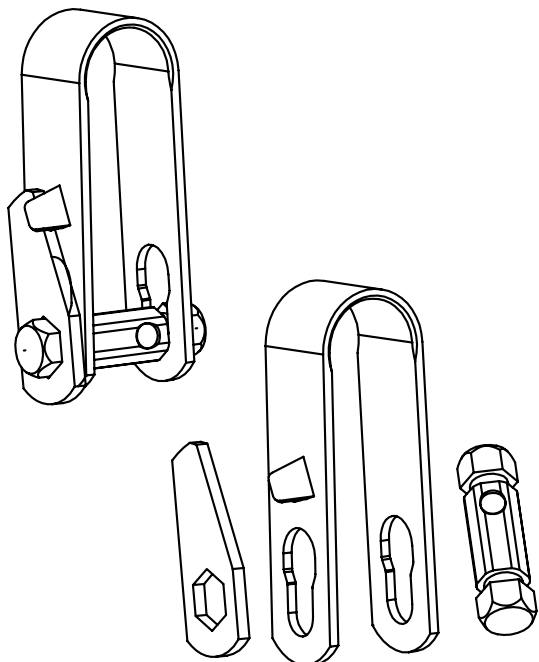
TIGHTENING HOOK "LIGHT"
