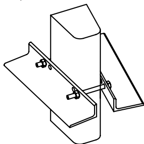
ANTI-SINKING PLATES (COUPLE INCLUDED FASTENERS AND NUTS M10)
