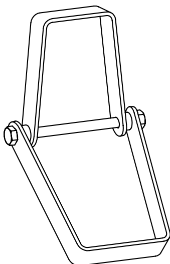
DOUBLE COLLAR FOR CONCRETE POST 7X7 AND 9X9
