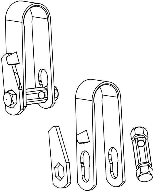
TIGHTENING HOOK "LIGHT"
